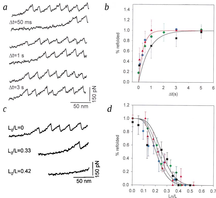
Fig. 3 Refolding kinetics of the I27 polyproteins. a , Unfolding and refolding cycles for a single V11P polyprotein. The protein was first stretched to almost its contour length to count the number of domains that unfolded ( N_{\text{total}} ) and then it was relaxed to its initial length to allow refolding. A second extension after a delay ( \Delta t ) measured the number of domains that refolded ( N_{\text{refolded}} ). b , Plot of the fraction of refolded domains, N_{\text{refolded}} / N_{\text{total}} versus \Delta t . The mutant polyproteins all refolded faster than the wild type. The solid lines are fits of the data to the single exponential function P_i(t) = 1 - e^{-t/\beta} ; the refolding rate \beta = 1.2 \text{ s}^{-1} for wild type (black line) and \beta = 2.8 \text{ s}^{-1} for the mutants (red line). c , The extent of refolding of a polyprotein depends on its residual tension. A polyprotein is first stretched to count the number of domains that unfold ( N_{\text{total}} ) and is then rapidly relaxed to a length L_0 for a fixed period of 5 seconds. L_0 / L (where L is the contour length) determines the residual force applied to the protein during refolding 32 . A second extension measures the number of domains that refolded under the residual tension ( N_{\text{refolded}} ). d , Plot of N_{\text{refolded}} / N_{\text{total}} versus L_0 / L . The black solid lines correspond to the Monte Carlo simulations with folding distances \Delta x_f = 2.0, 2.3 and 2.6 \text{ nm} (from left to right).
